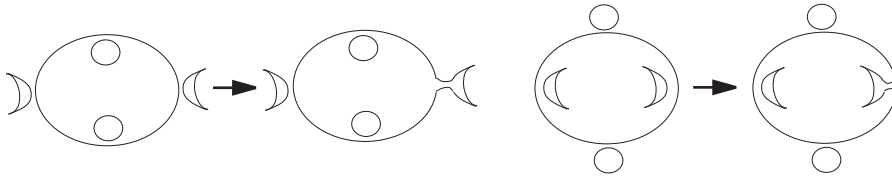
FIGURE 7. Fusion moves
