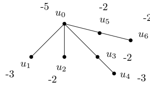
FIGURE 3. The configuration Q
