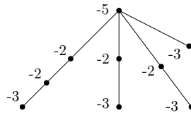
FIGURE 7. The configuration \mathcal{U}
