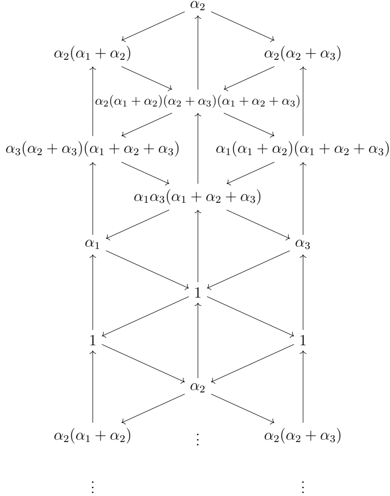
FIGURE 2. Values of \tilde{D}_\xi^{-1} on the cluster variables of the seed \mathcal{S}^{\hat{1}_Q} of \mathcal{A}^{\leq \xi} in type A_3 .
