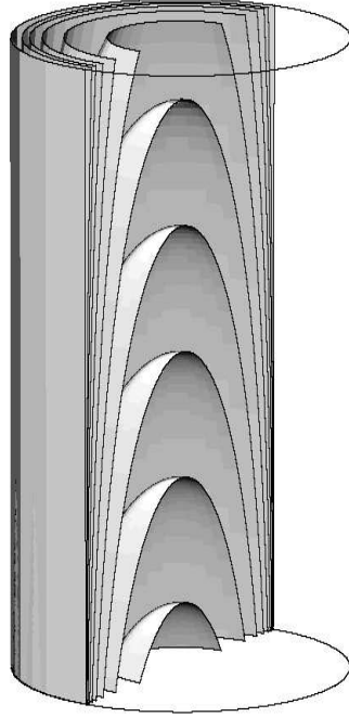
FIGURE 3. The Reeb foliation
