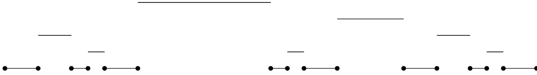
FIGURE 13. The Fibonacci Cantor set.
