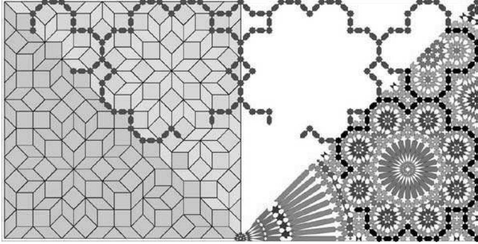
FIGURE 10. Quasiperiodic tilings and zellijis.
