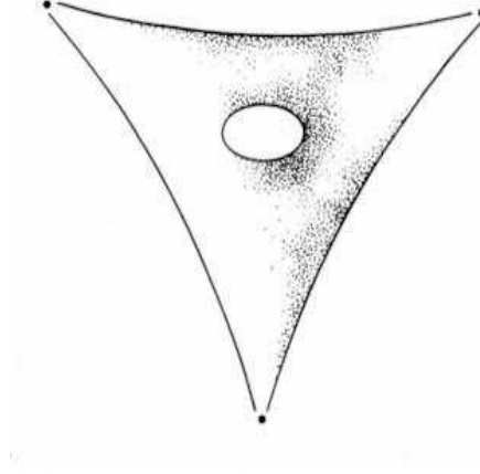
FIGURE 8. Hyperbolic orbifolds.
