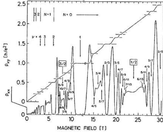
FIGURE 7. Observed fractions in the quantum Hall effect.
