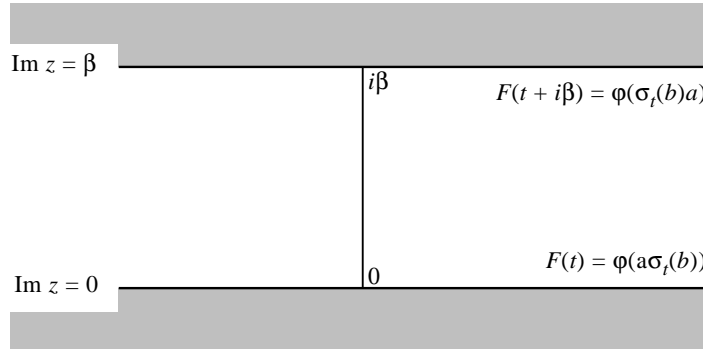
FIGURE 1. The KMS condition
