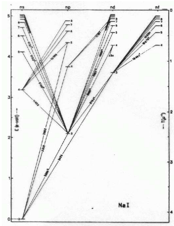
FIGURE 2. Spectral lines and the Ritz-Rydberg law.
