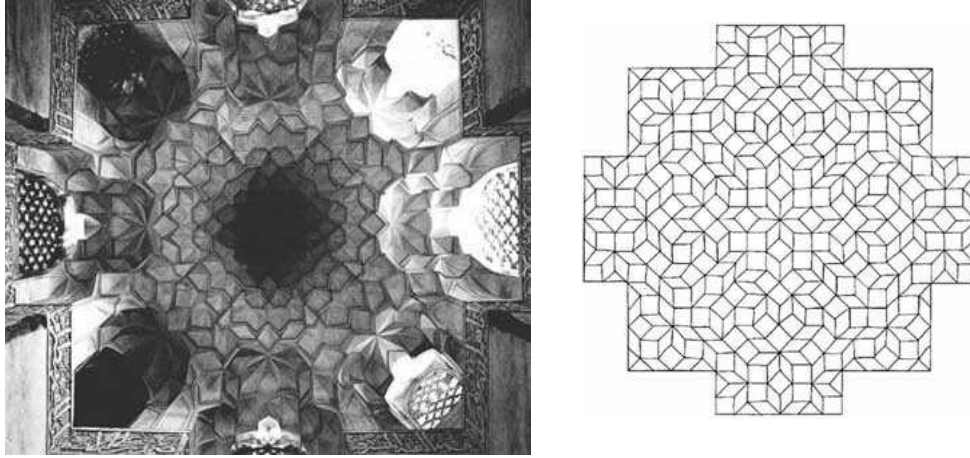
FIGURE 11. Quasiperiodic tilings and muqarnas.
