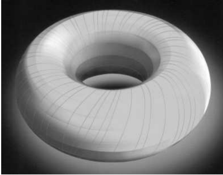
FIGURE 4. The Kronecker foliation and the noncommutative torus
