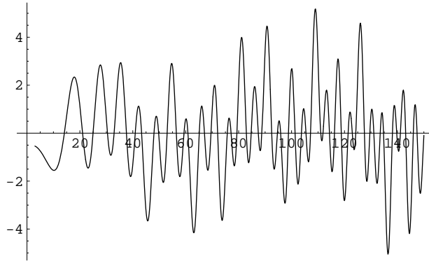
FIGURE 18. Zeros of zeta
