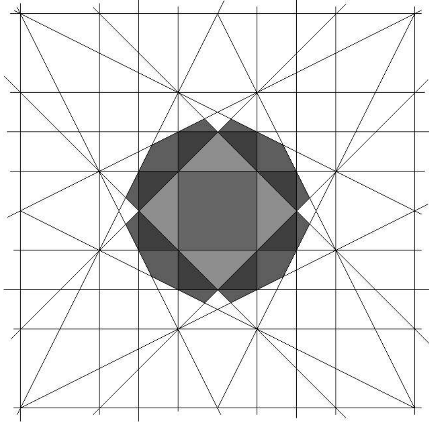
FIGURE 6. Brillouin zones for a 2-dimensional crystal
