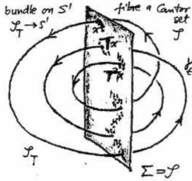
FIGURE 12. Mapping Torus
