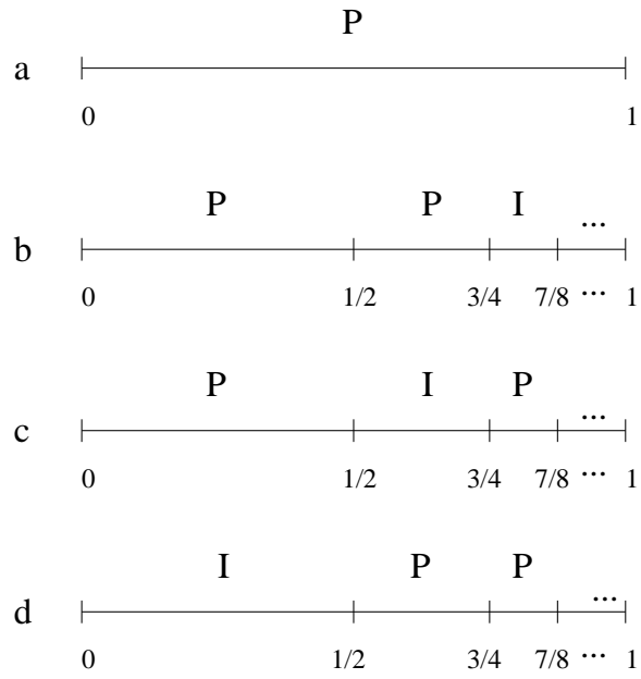
Figure 2: Action on the interval [0, 1]
