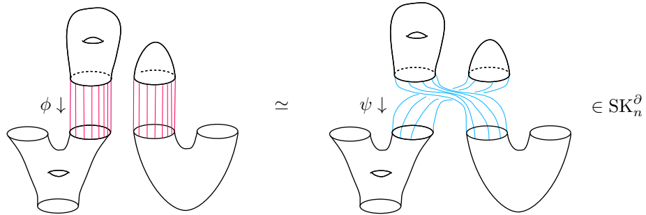
FIGURE 3. Example of an SK_n^\partial -relation
