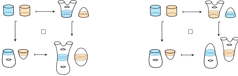
FIGURE 6. Two examples of distinguished squares
