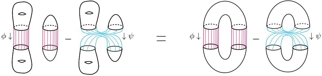
FIGURE 5. Example of an SKK-relation
