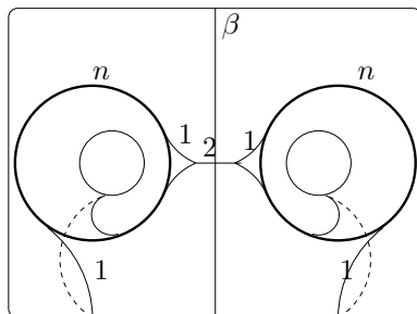
FIGURE 3. An example of a train track \tau needed in the proof of Lemma 2.13. The symmetric multicurve \alpha^d is represented in thick lines. The weights for \alpha_n^d on the various branches are indicated.
