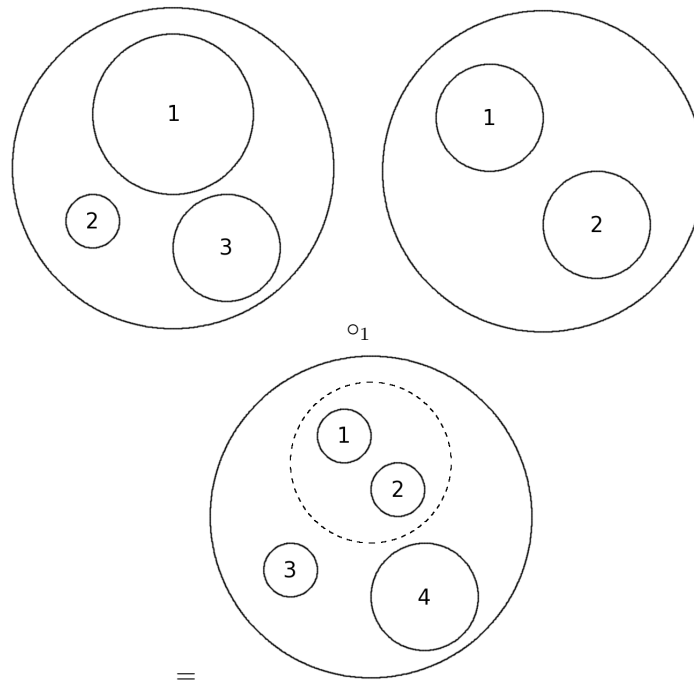
FIGURE 3. Exemple of partial composition in the little discs operad
