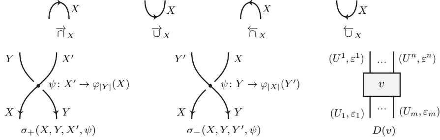
FIGURE 4. Elementary colored diagrams
