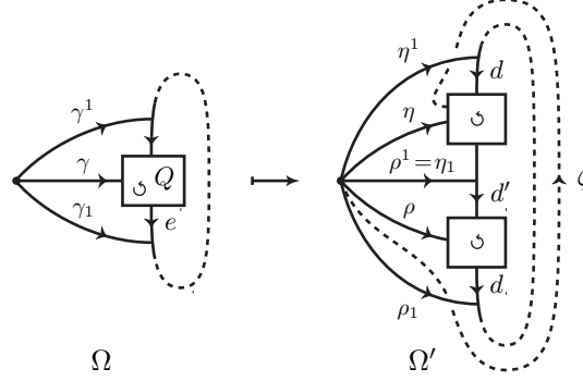
FIGURE 12. The ribbon graphs \Omega and \Omega'
