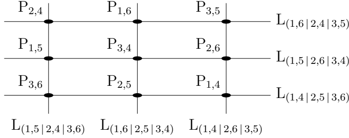
FIGURE 1. The jail subconfiguration CR'_{\{1,2,3\},\{4,5,6\}} in the Cremona–Richmond configuration CR
