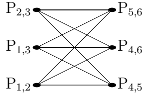
FIGURE 2. The bipartite subconfiguration CR''_{\{1,2,3\},\{4,5,6\}} in the Cremona–Richmond configuration CR
