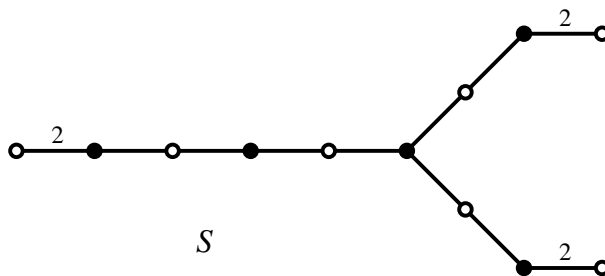
Figure 24: Tree S
