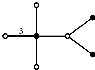
Figure 26: This tree also has monodromy group \mathrm{PGL}_2(7) .
