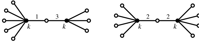
Figure 34: Two trees with the passport (k^2, 4^1 1^{2k-4}) . One of them is symmetric, the other one is not.
