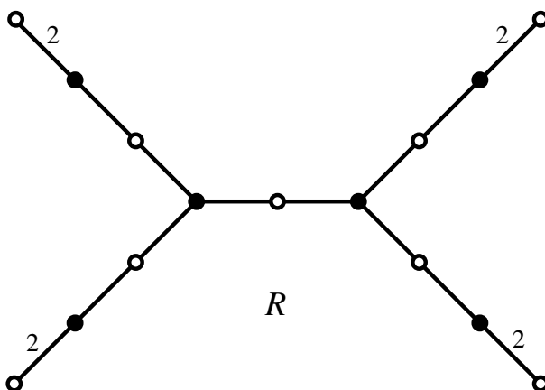
Figure 23: Tree R
