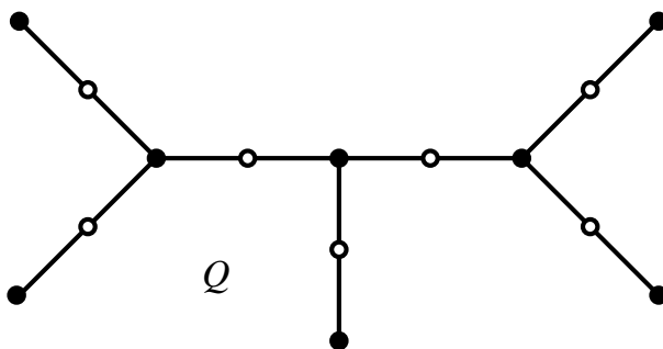
Figure 22: Tree Q
