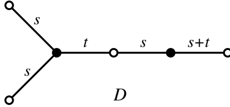
Figure 4: Fork-trees. There are exactly two leaves of weight s and exactly one leaf of weight s + t . As usual, \gcd(s, t) = 1 .
