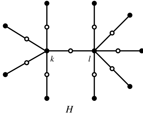
Figure 11: Series H : ordinary trees of diameter 6 which are decomposable.
