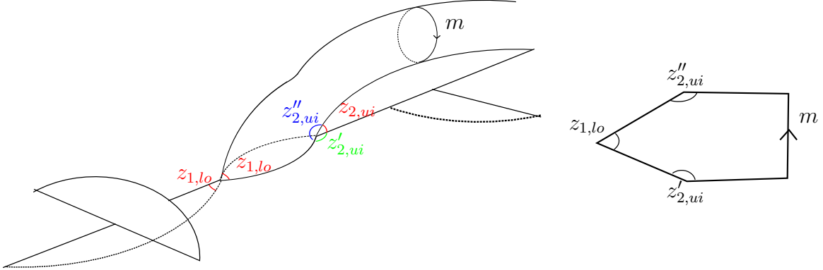
FIGURE 7. The meridian positioned on top of overpass 2, and the left part of the region of the 5t spine that m intersects.
