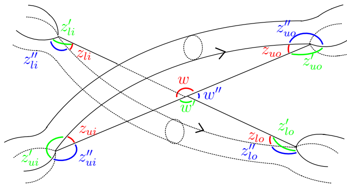
FIGURE 4. The 5T-spine near a crossing of D , and the shape parameters of each corner of the spine. The arrows specify the orientation of strands.
