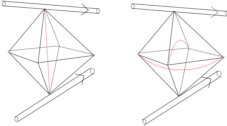
FIGURE 3. Any octahedron can be split into 4 or 5 tetrahedra by adding the red dashed edges to it.
