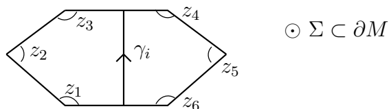
FIGURE 2. A segment \gamma_i of a peripheral loop \gamma intersecting a region of the spine. The boundary component \Sigma to which \gamma belongs lies above the region. In this example, h_{\gamma_i} = -z_1 z_2 z_3 = -\frac{1}{z_4 z_5 z_6} .
