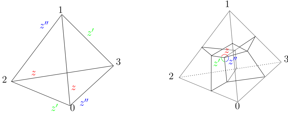
FIGURE 1. The dual spine to the triangulation and the shape parameters associated to corners of the spine.
