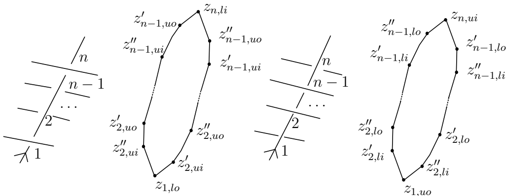
FIGURE 5. An overarc (resp. underarc) and the corresponding upper (resp. lower) shingle region of the spine, with shape parameters.
