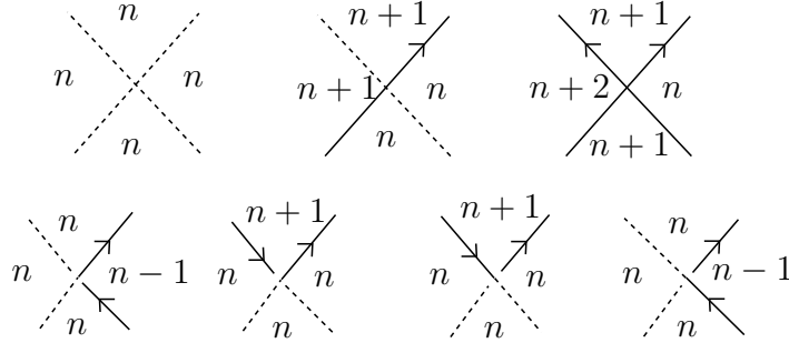
FIGURE 10. The local pattern of winding numbers near a crossing. Strands of \gamma are represented by solid lines, strands of \gamma' by dashed lines. The bottom row corresponds to the 4 different possibilities for over/underpass j : positive overpass, negative overpass, positive underpass, or negative underpass.
