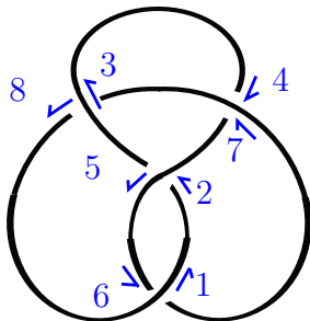
FIGURE 9. A labelling of the crossings of a Figure eight knot diagram. The 4 distinct crossings of the diagram have labels (1, 6) , (2, 5) , (3, 8) and (4, 7) .
