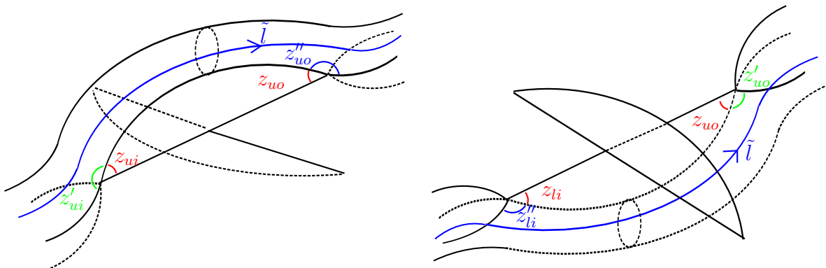
FIGURE 8. The longitude \tilde{l} on the 5t -spine, and the shape parameters to the left (resp. to the right) of it on overpasses (resp. underpasses).
