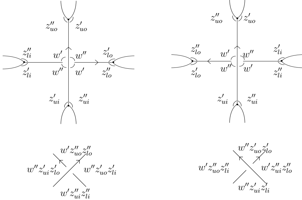
FIGURE 6. On the top, a top view of the 5t -spine near a positive and a negative crossing. On the bottom, the rule describing the corner factors.
