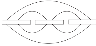
FIGURE 14. Theta networks turn into Ext groups or even Ext algebras of simple objects.
