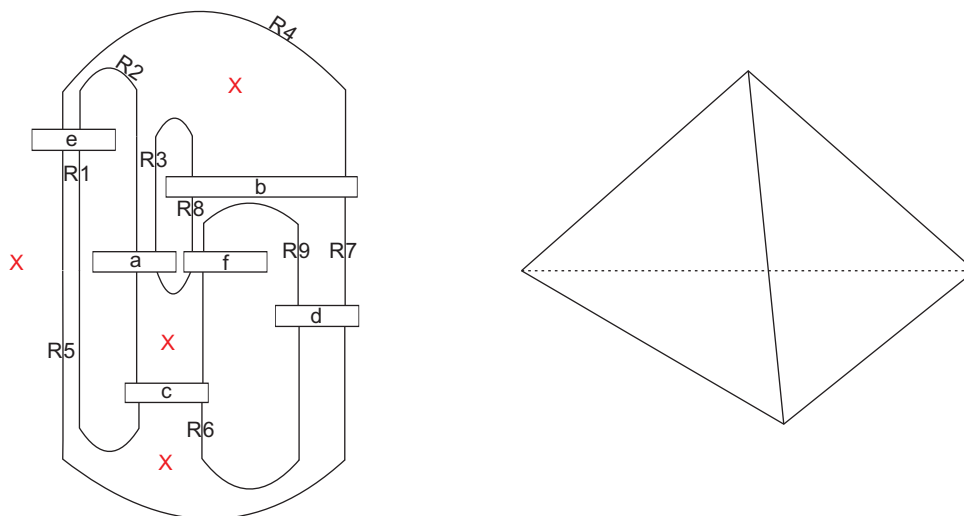
FIGURE 15. The tetrahedron network (the numbers indicate that there are that many copies of the strand). The Jones-Wenzl projectors correspond to the 6 vertices of the tetrahedron.
