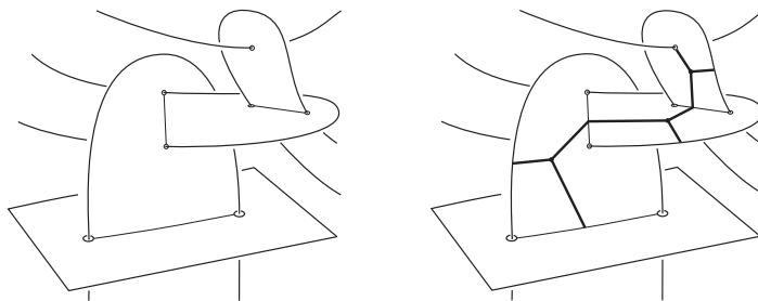
FIGURE 3. Part of a Whitney tower in 4-space (left), and shown with part of an associated tree (right). Whitney disks pair up transverse intersections of opposite sign.
