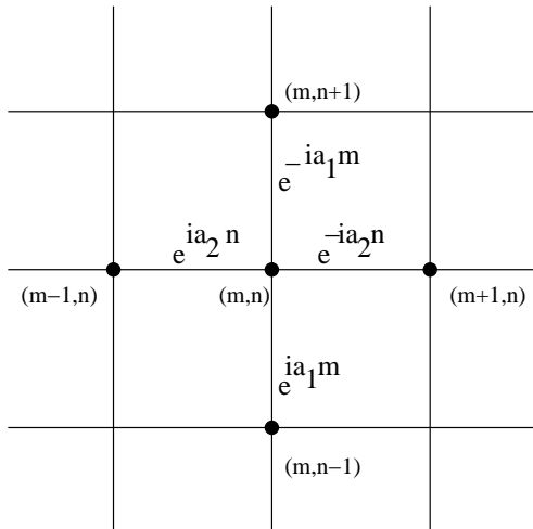
FIGURE 7. The Harper operator on the square lattice
