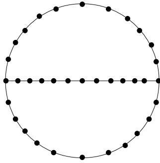
FIGURE 2. The graph H(\Lambda_\Gamma)/\Gamma for t = \pi^5 in Kato's family.
