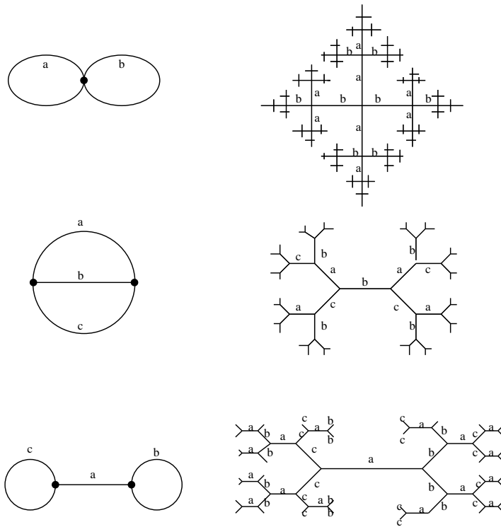
FIGURE 1. The graphs \mathcal{T}_\Gamma/\Gamma for genus g = 2 , and the corresponding trees \mathcal{T}_\Gamma .
