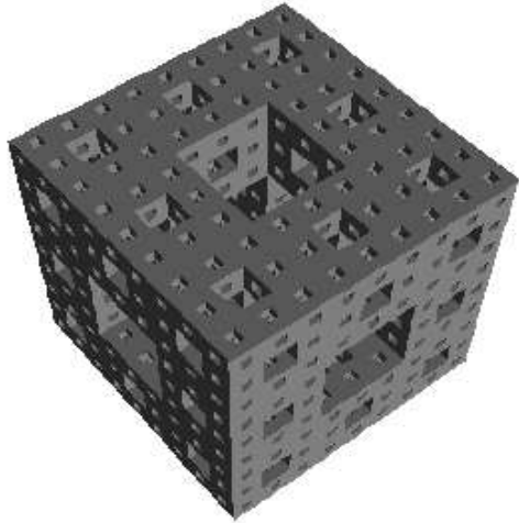
FIGURE 3. The universal Menger curve (iterative construction).
