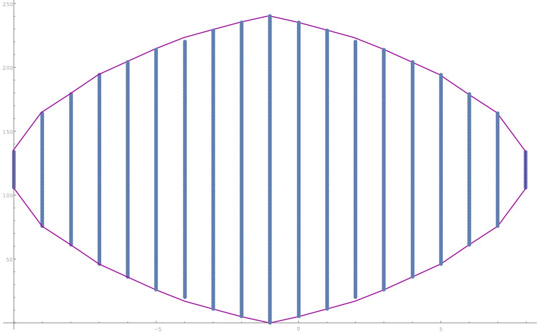
Figure 11: The Newton polygon of the Toda spectral curve for \mathcal{G}^\# = E_8^\# and \rho = 248 .
