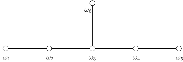
Figure 6: The Dynkin diagram of \mathcal{G} = E_6 . Nodes in the diagram are labeled by the corresponding fundamental weights; we have \rho_{\min} \triangleq \rho_{\omega_1} = \mathbf{27} = \overline{\rho_{\omega_5}} , \rho_{\omega_2} = \Lambda^2 \rho_{\omega_1} = \mathbf{351} = \overline{\rho_{\omega_4}} , \rho_{\omega_3} = \Lambda^3 \rho_{\omega_1} = \mathbf{2925} , \rho_{\omega_6} = \text{Adj} = \mathbf{78} .
