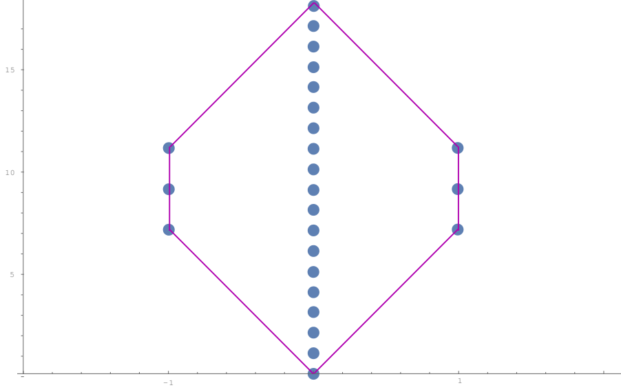
Figure 5: The Newton polygon of the Toda curve for \mathcal{G} = D_{p+2} , minimal representation \rho_{\omega_1} = \mathbf{2(p+2)}_{\mathbf{v}} for p+2 = 9 .
