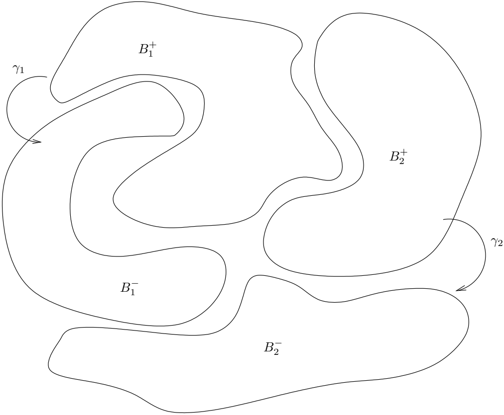
FIGURE 1. A Schottky group.
