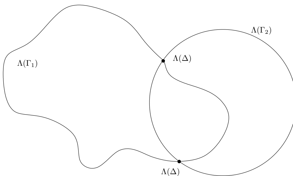
FIGURE 3. Combination of two 1-quasifuchsian groups: \Gamma = \Gamma_1 *_Z \Gamma_2 .
