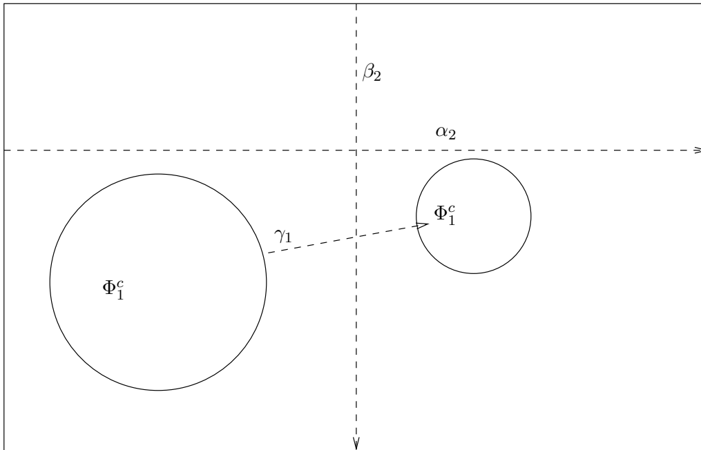
FIGURE 2. A classical Schottky-type group. It is isomorphic to \mathbb{Z} * \mathbb{Z}^2 with \mathbb{Z} = \langle \gamma_1 \rangle , \mathbb{Z}^2 = \langle \alpha_2, \beta_2 \rangle .
