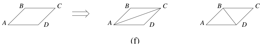
Figure 4: Degenerate second bifurcations
