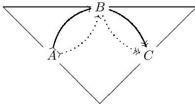
FIGURE 1. Nenashev's representative of an element in K_1\mathbf{E} .
