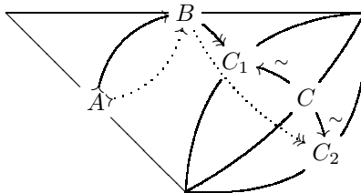
FIGURE 2. Our representative of an element in K_1\mathbf{W} .
