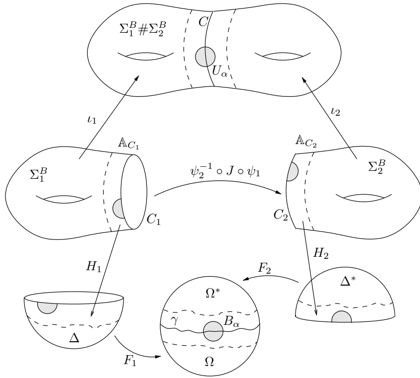
FIGURE 3.1. Sewing using quasisymmetric boundary identification.
