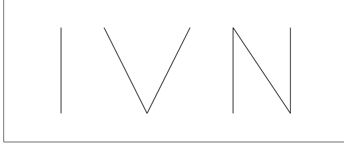
FIGURE 3. Three complexes: one with all vertices exchangeable; one with some vertices but not all exchangeable; and one with no vertices exchangeable.
