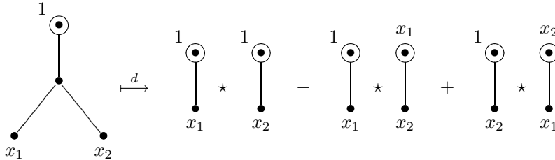
Figure 4: The differential on a tree with one internal vertex.
