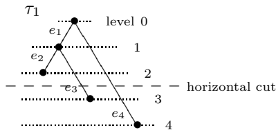
A horizontal cut of the level tree \tau_1 with edge sequence (e_3, e_4) .
