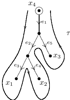
Figure 1: An R -deco tree \tau with root vertex decorated by x_4 .
