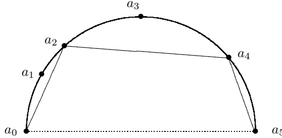
A 4-gon for the subsequence (a_2, a_4) of (a_1, \dots, a_4) inscribed in the semicircle
