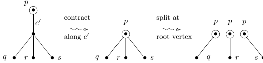
Figure 3: Contracting the root edge.
