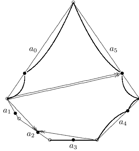
The picture after pushing arrows inside.
