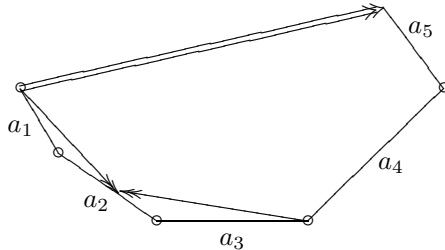
A dissection associated to the term I(a_0; a_2, a_4; a_5) \otimes I(0; a_1; a_2)I(0; a_3; a_2) .
