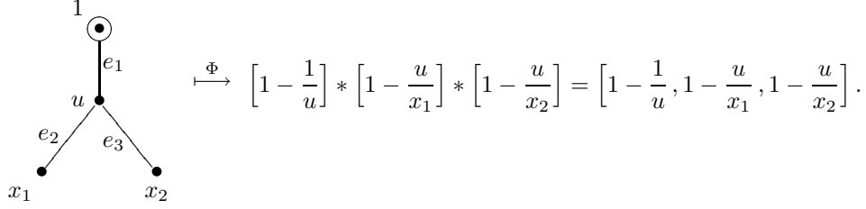
Figure 5: The forest cycling map on a tree with one internal vertex.
