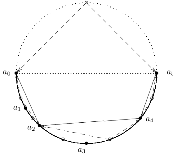
An 8-gon circumscribing the 4-gon (a_0, a_2, a_4, a_5) inscribed in the semicircle
