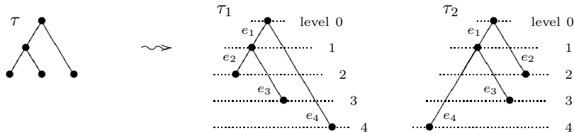
A tree \tau , and two of its eight level trees, denoted \tau_1 and \tau_2 .
