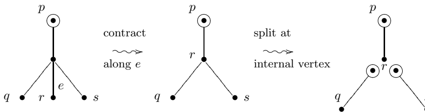
Figure 2: Contracting a leaf.
